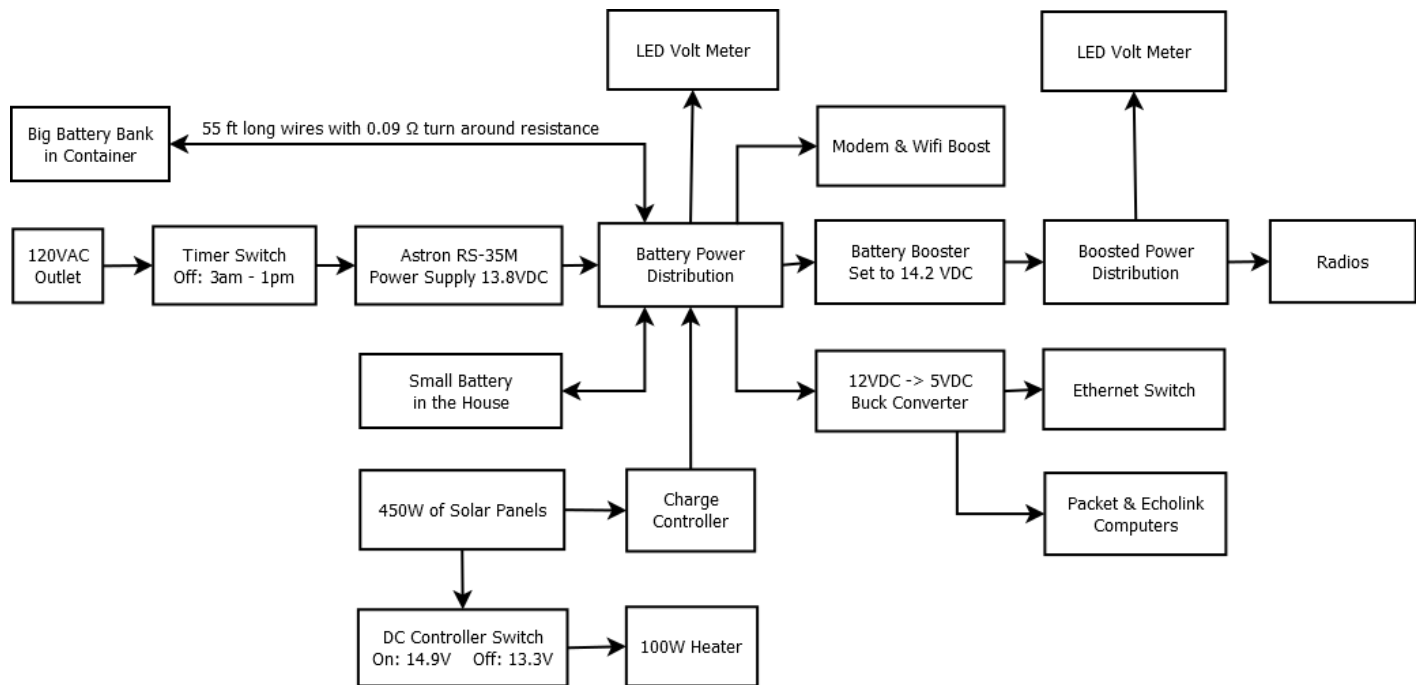
VA7FI's setup. The direction of the arrow indicates direction of power.
