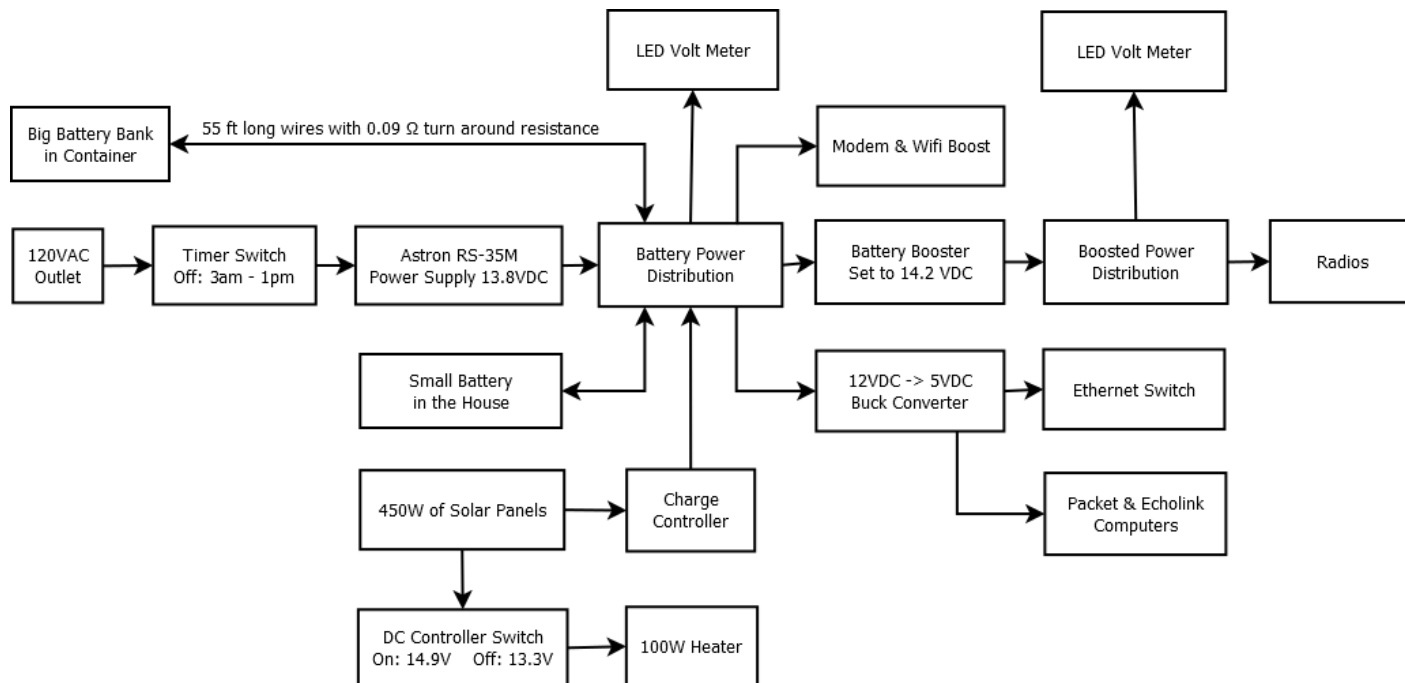
VA7FI's setup. The direction of the arrow indicates direction of power flow.
