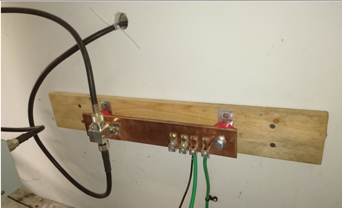
The grounding bar connects to the main ground in the communication cabinet.
